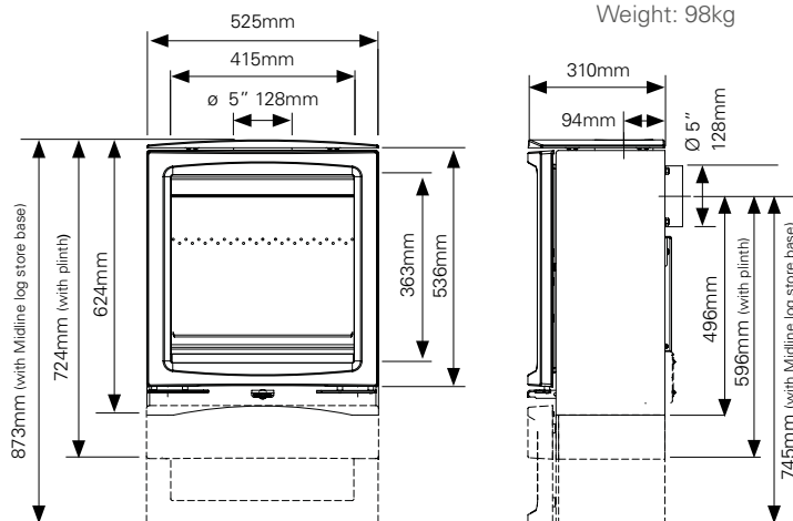
Vogue Midi T woodburning Ecodesign stove with optional Midline wood store base.
